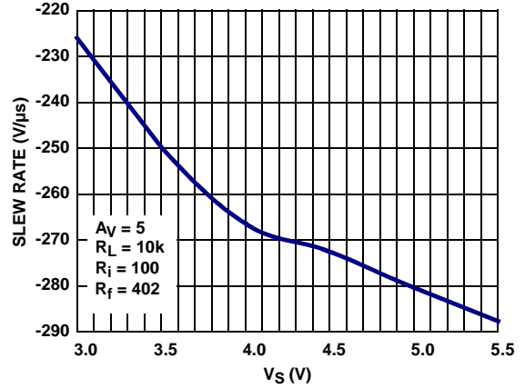
FIGURE 28. ISL55290 NEGATIVE SLEW RATE vs VS
